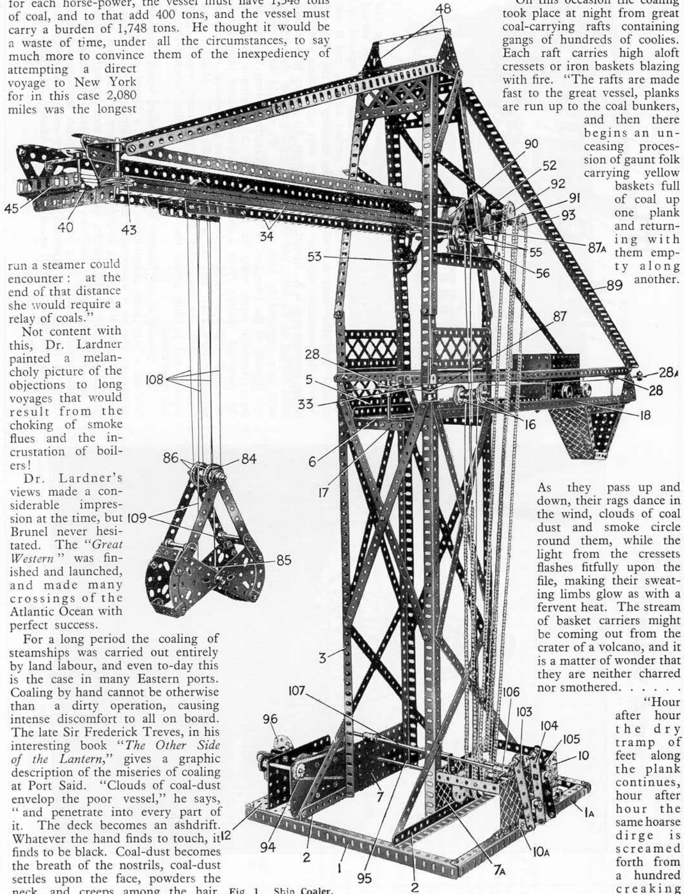
Fig. 1. Ship Coaler.
