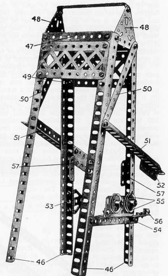
Fig. 3. Upper Portion of Tower
