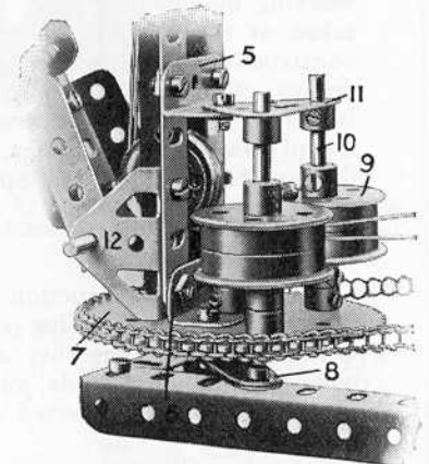
Fig. 4. Swivelling base of Jib.
