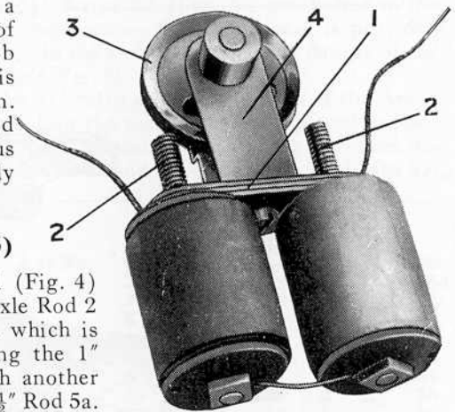
Fig. 3. The Meccano Electro Magnet.
