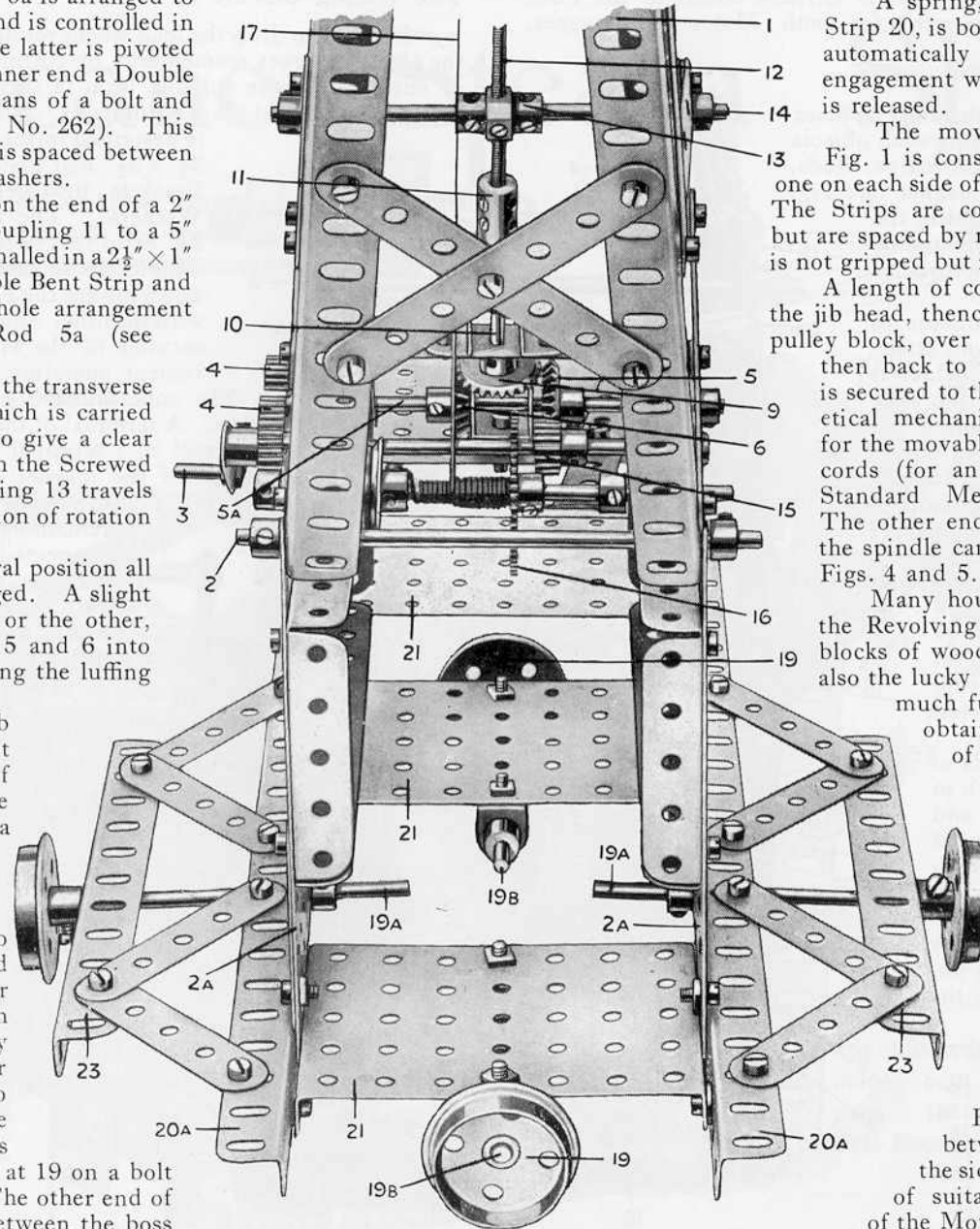
Fig. 4. Front view of Crane, showing hoisting mechanism, etc.
