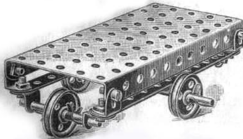
Fig. 3. Revolver Truck
