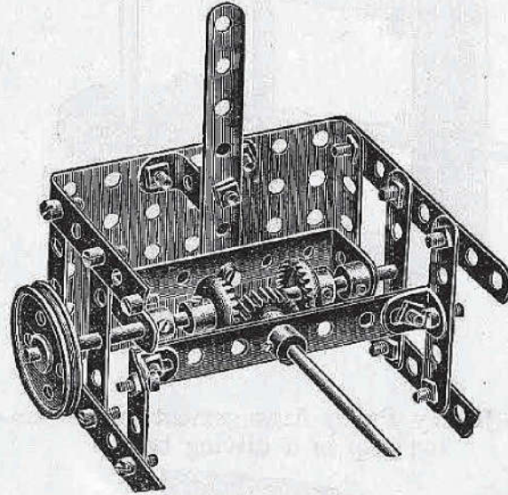
F —Spring controlled Band Friction Brake.
