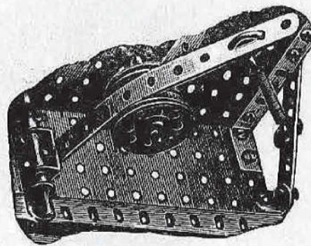
F —Spring controlled Band Friction Brake.
