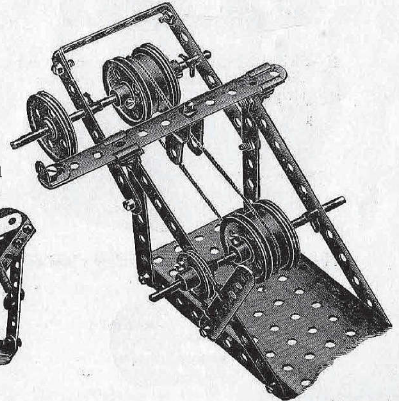
G —Method of operating a fast and loose pulley with a belt drive, one of the flanged wheels on the main shaft being secured whilst the other runs freely.
