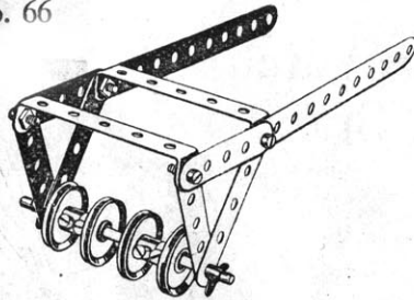
Furrowing Roller
