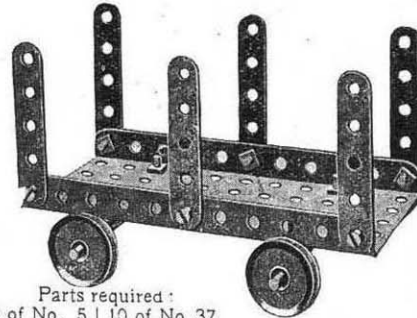
Model No. 9 - Timber Truck
