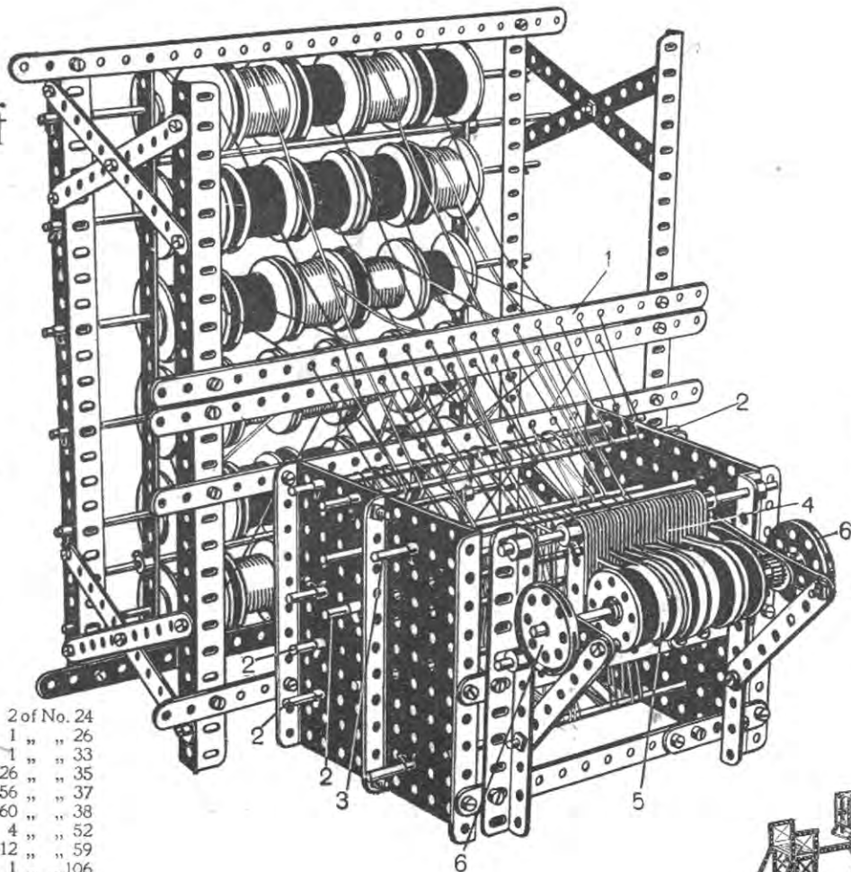
No. 319. Beaming Frame.
