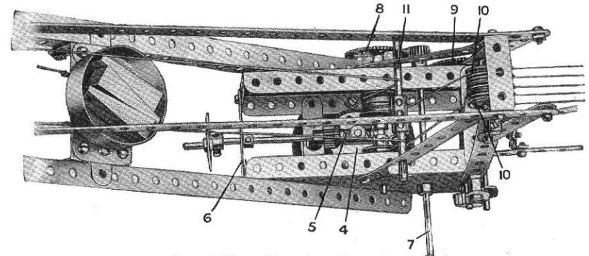
FIG. 4.45A. Plan view of gear box.
