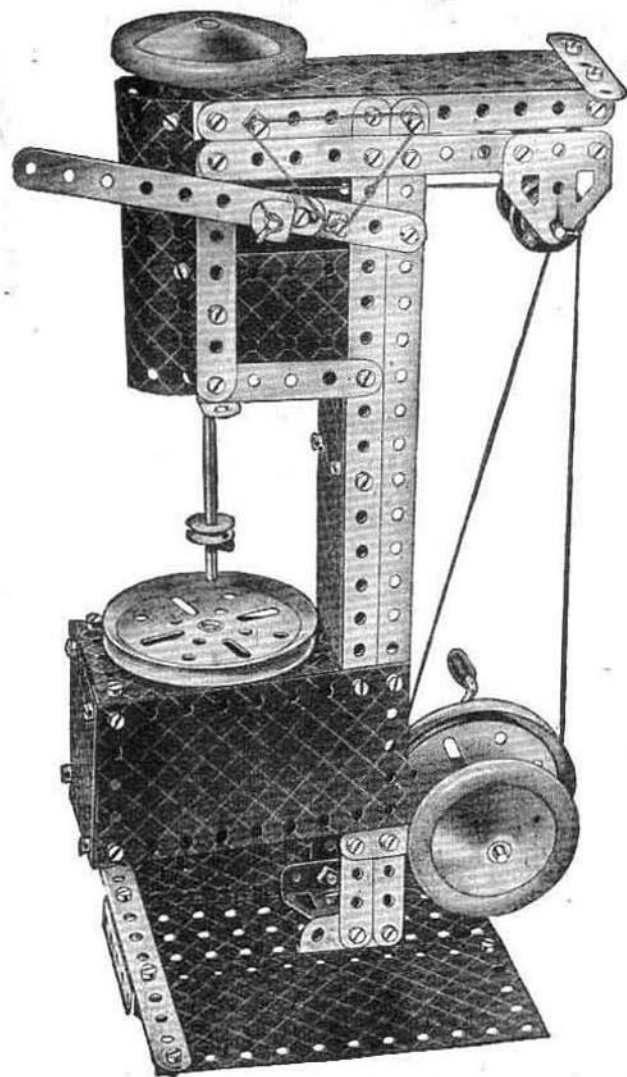
Drilling Machine
