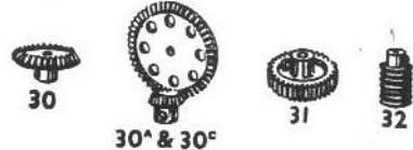
30. Bevel Gear, 3/4" diam., 26 teeth (for use in pairs) 30a. Bevel Gear, 1/2" diam., 16 teeth } Can only be used together 30c. Bevel Gear, 1 1/2" diam., 48 teeth } 31. Gear Wheel, 1 1/2" diam., 1/4" face, 38 teeth 32. Worm, 1/2" diam. 34. Spanner
