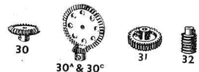
30. Bevel Gear, 1" diam., 26 teeth (for use in pairs) 30a. Bevel Gear, 1" diam., 16 teeth | Can only be used together 31. Gear Wheel, 1" diam., 4" face, 38 teeth 32. Worm, 1" diam. 34. Spanner
