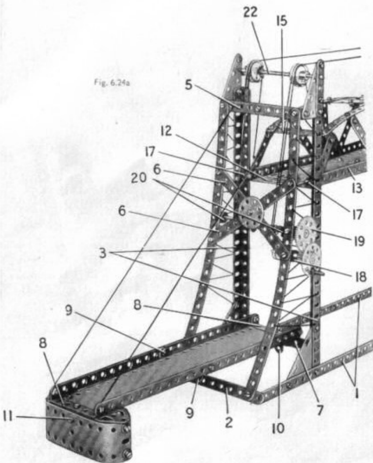
MODEL 6.24 LIFTING BRIDGE — Continued
