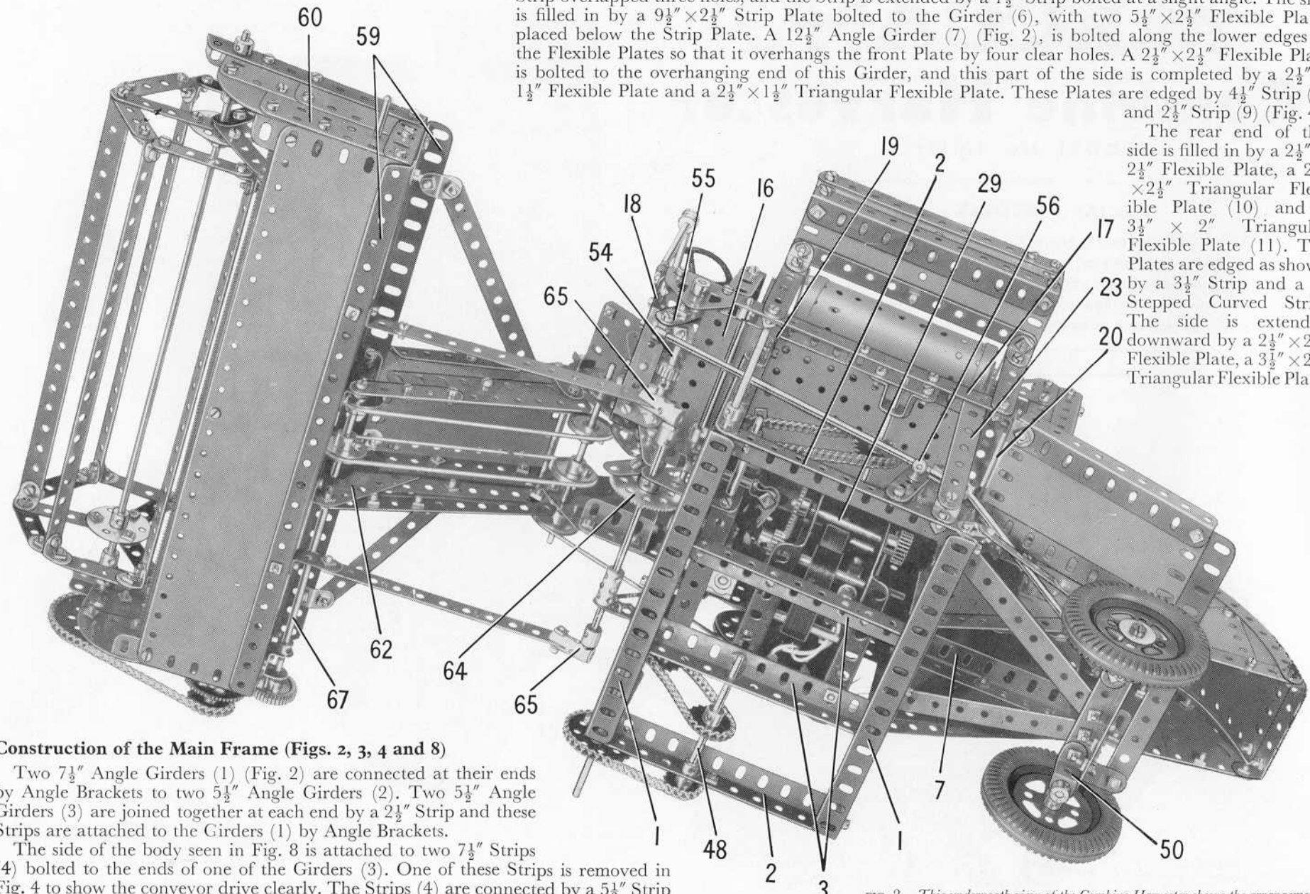
FIG. 2 This underneath view of the Combine Harvester shows the arrangement of the conveyor, the underframe and the steering mechanism
