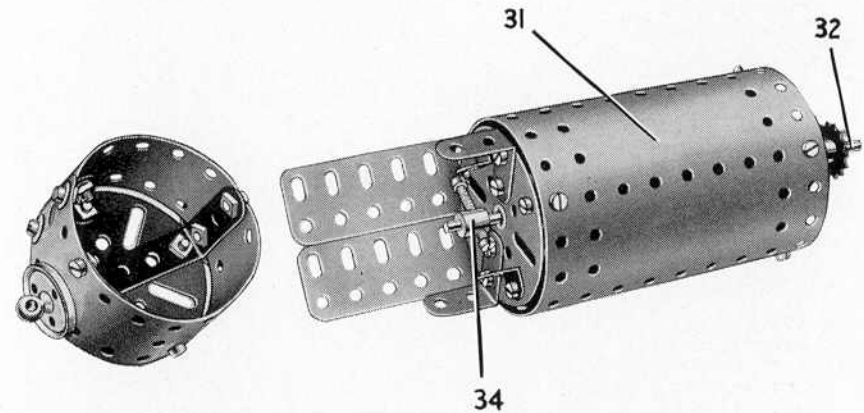
FIG. 9 The magneto, with the cap shown separately
