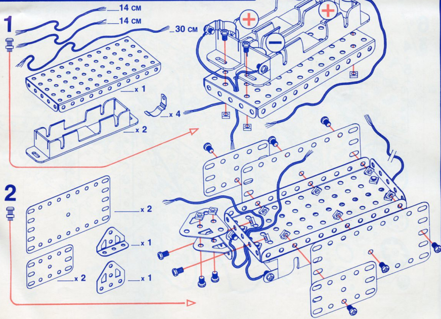
Fork-lift truck Chariot élévateur Hubstapler Hefttruck Carrello elevatore Carro elevador
